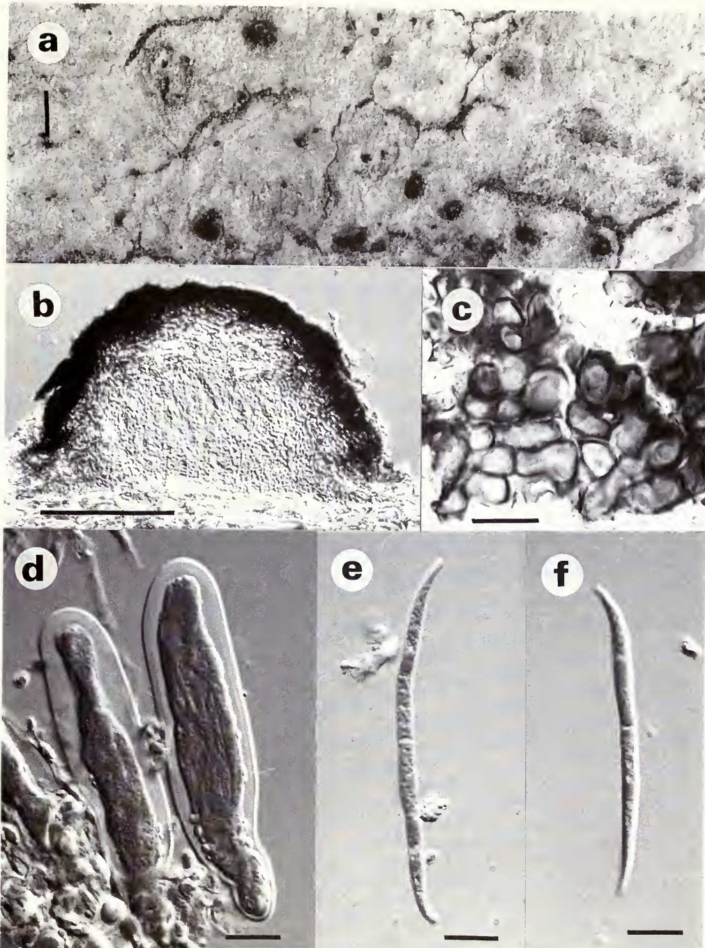
Fig. 12 Leptorhaphis lucida Körber (L-Körper Lich. Sel. Germ. exs. no. 262) (a) Surface view; scale = 500 \mu m; (b) Vertical section of ascoma; scale = 100 \mu m; (c) Detail of involucrellum (surface view): textura globulosa; (d) Asci; (e), (f) Ascospores; scale = 10 \mu m.
